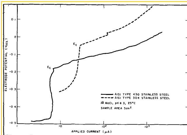
Fig. 1. Potentiodynamic anodic-polarization curves for steels exposed to hydrogen-saturated 1M NaCl sweep rate, 0.600 V/hr
