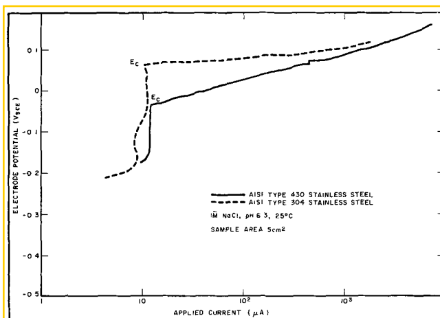
Fig. 3. Potentiodynamic anodic-polarization curves for steels exposed to oxygen-saturated 1M NaCl sweep rate, 0.600 V/hr.
